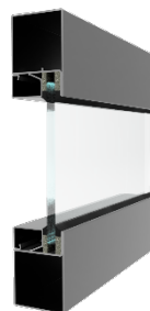
Typical Screen
