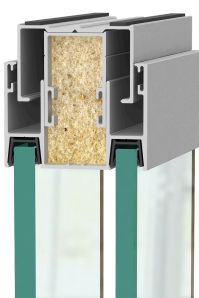
3-Part +/- 25mm deflection head
