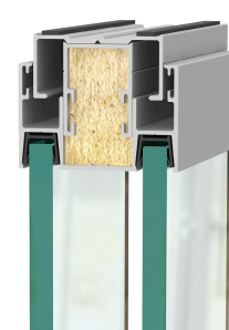
2-Part +/- 15mm deflection head
