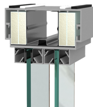
Double glazed module
