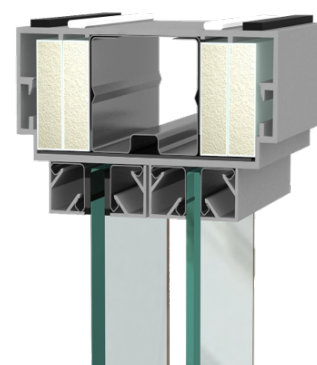
Double glazed module
