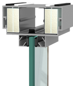
Single centre glazed module
