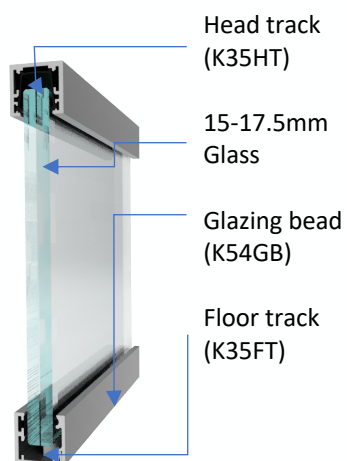
Standard Single Glazed Head and Base Detail
