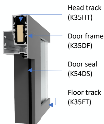
Standard Full Height Door Frame Detail
