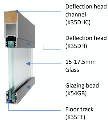
Standard +/-25mm Deflection Head and Base Detail
