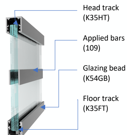
Single Glazed with Applied Kross Glaze Bars
